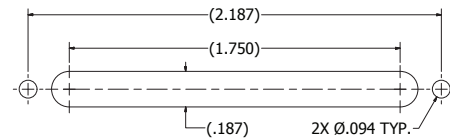
PANEL CUTOUT
