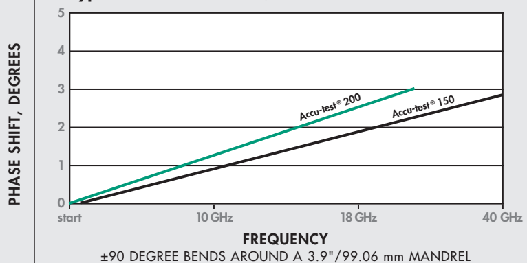
Typical Phase vs. Flexure, Accu-Test® 150 & 200 Cables
